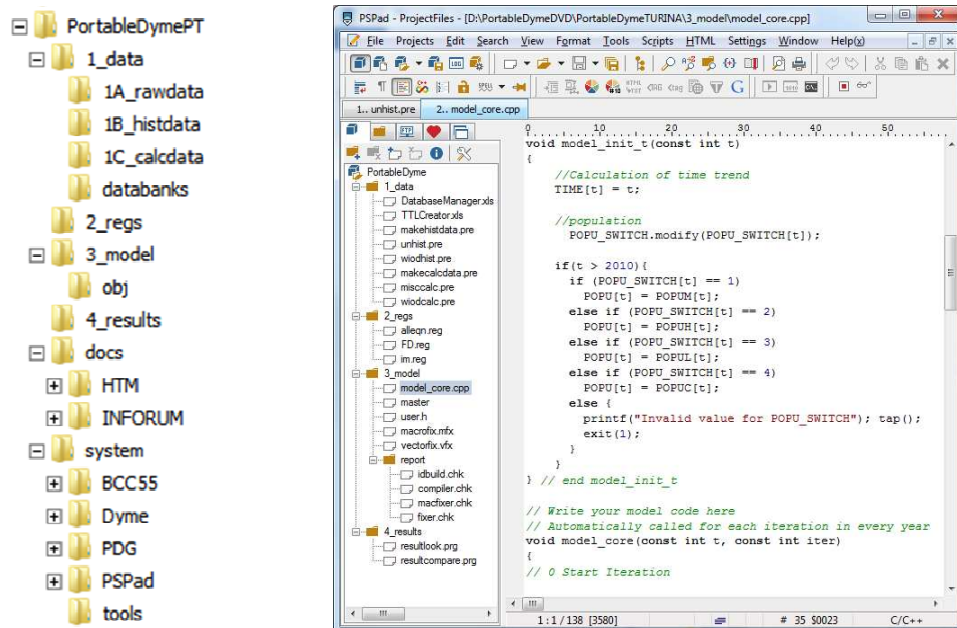
Figure 1. Structure of PortableDyme Models.
